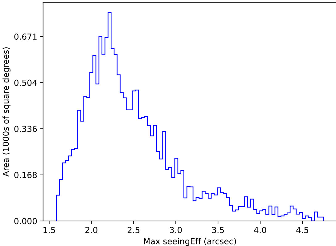
roll_pause_mjdp0_v3.4_10yrs WFD y band: Max seeingEff
