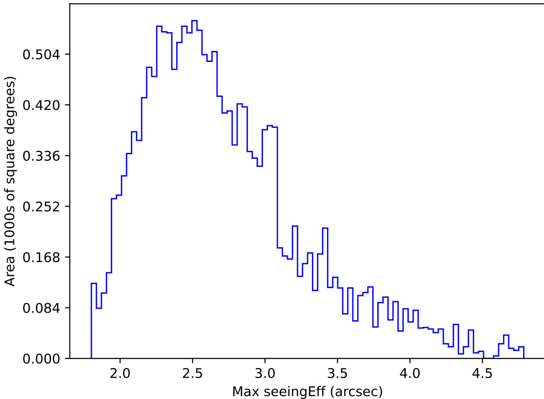
roll_pause_mjdp0_v3.4_10yrs WFD r band: Max seeingEff
