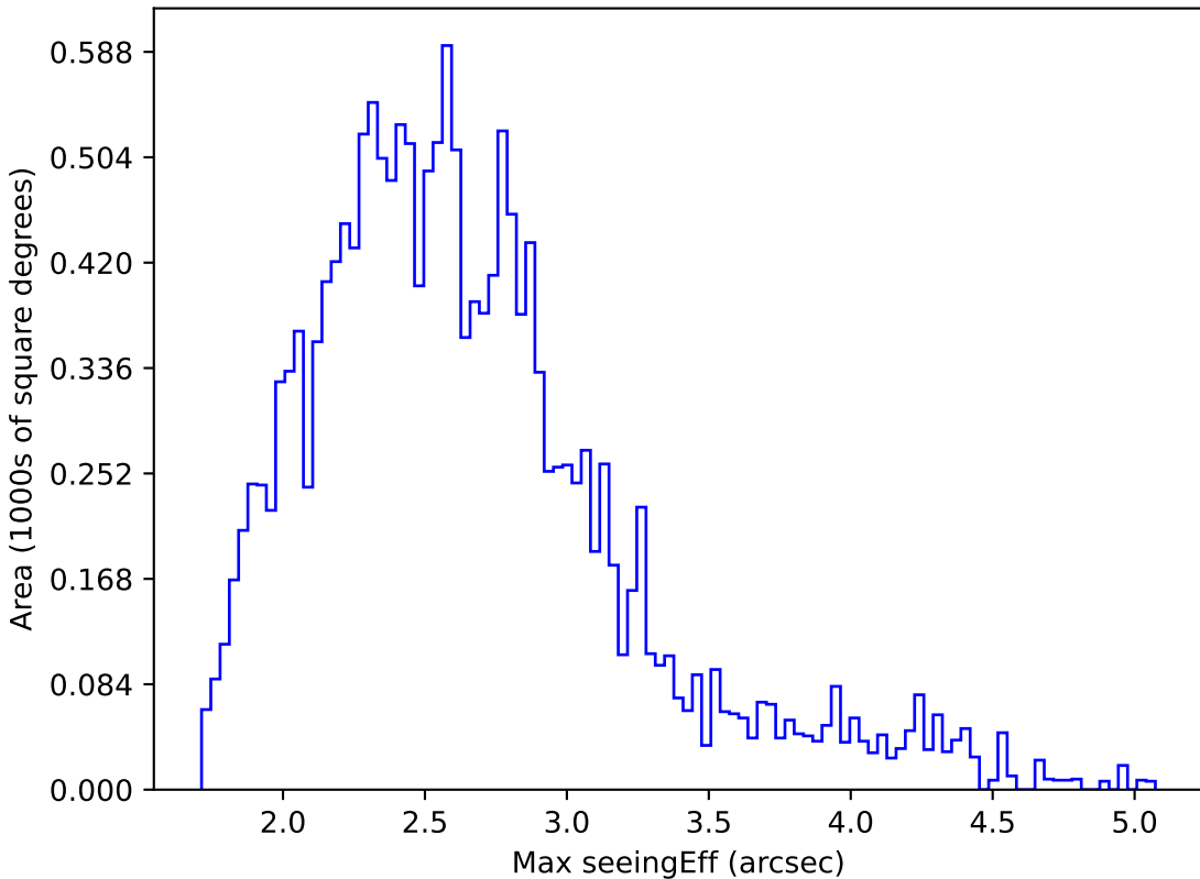
roll_pause_mjdp0_v3.4_10yrs WFD i band: Max seeingEff
