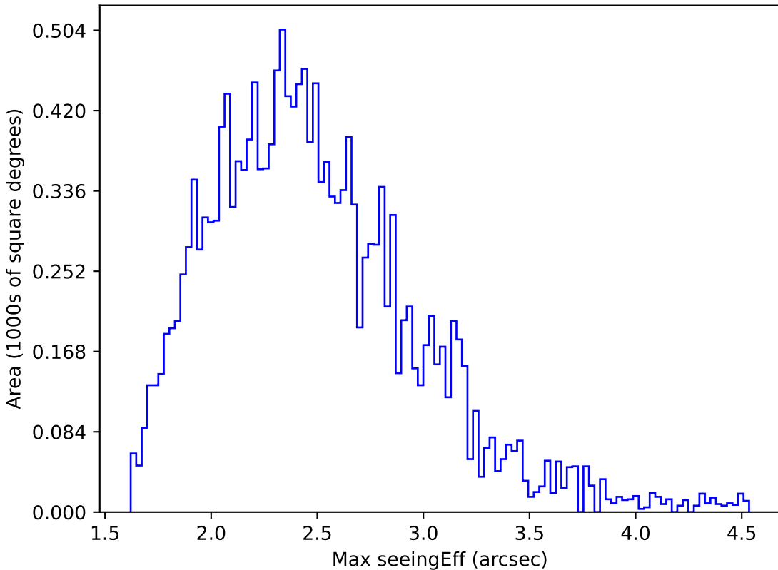
roll_pause_mjdp0_v3.4_10yrs WFD g band: Max seeingEff
