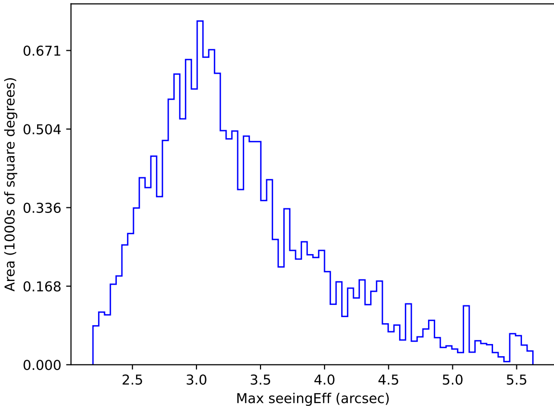
roll_pause_mjdp0_v3.4_10yrs WFD all bands: Max seeingEff
