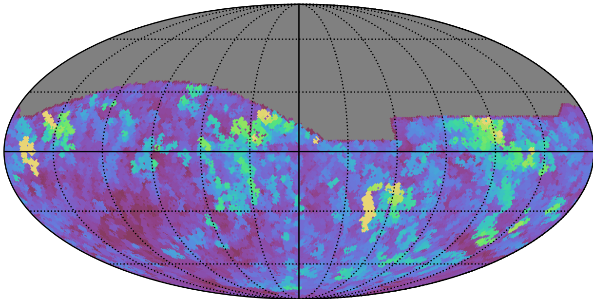
roll_pause_mjdp0_v3.4_10yrs All sky z band: Max seeingEff
