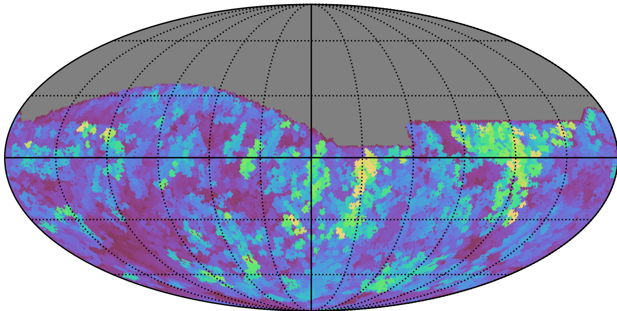
roll_pause_mjdp0_v3.4_10yrs All sky r band: Max seeingEff
