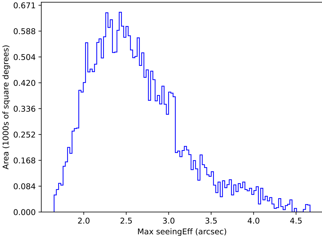
roll_pause_mjdp0_v3.4_10yrs All sky r band: Max seeingEff
