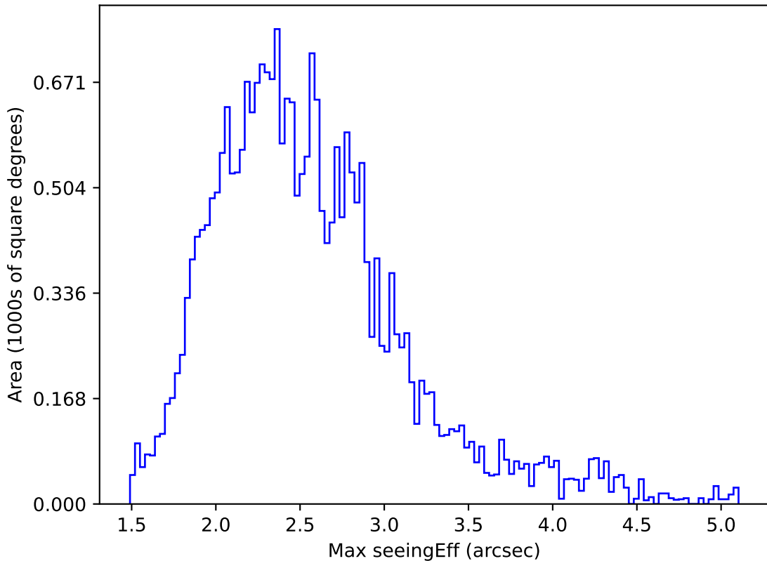
roll_pause_mjdp0_v3.4_10yrs All sky i band: Max seeingEff
