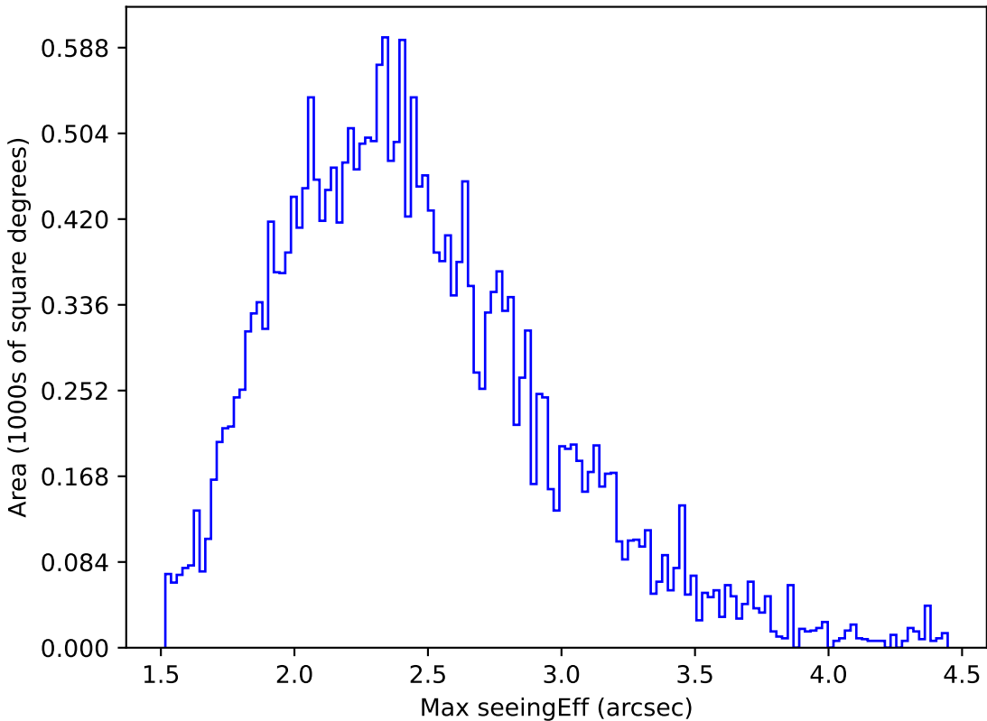
roll_pause_mjdp0_v3.4_10yrs All sky g band: Max seeingEff
