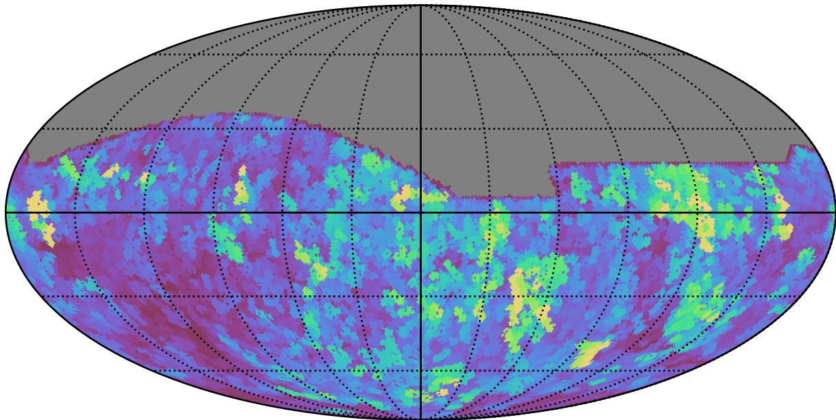
roll_pause_mjdp0_v3.4_10yrs All sky all bands: Max seeingEff
