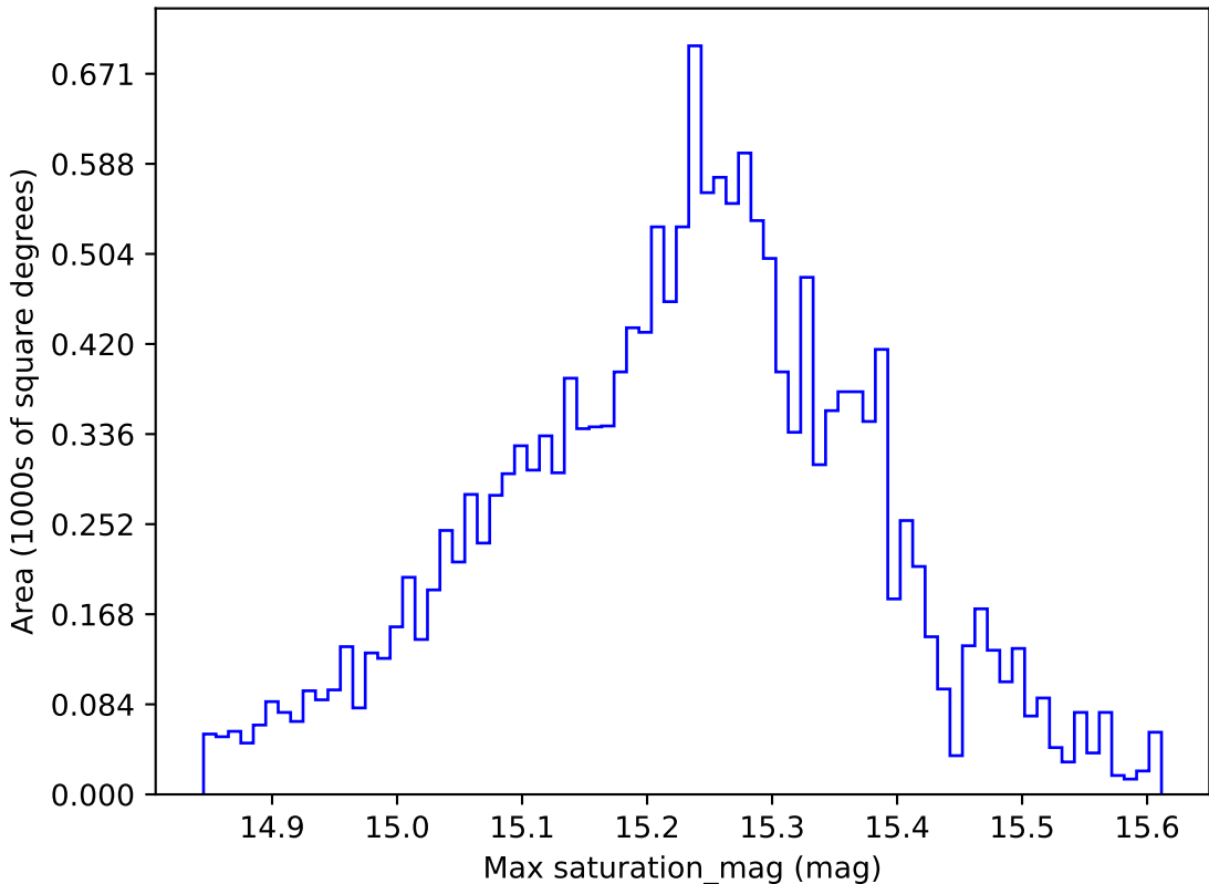
roll_pause_mjdp0_v3.4_10yrs WFD z band: Max saturation_mag
