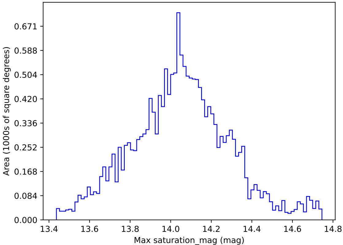
roll_pause_mjdp0_v3.4_10yrs WFD u band: Max saturation_mag
