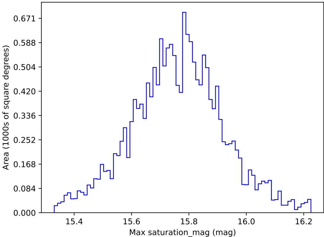
roll_pause_mjdp0_v3.4_10yrs WFD r band: Max saturation_mag
