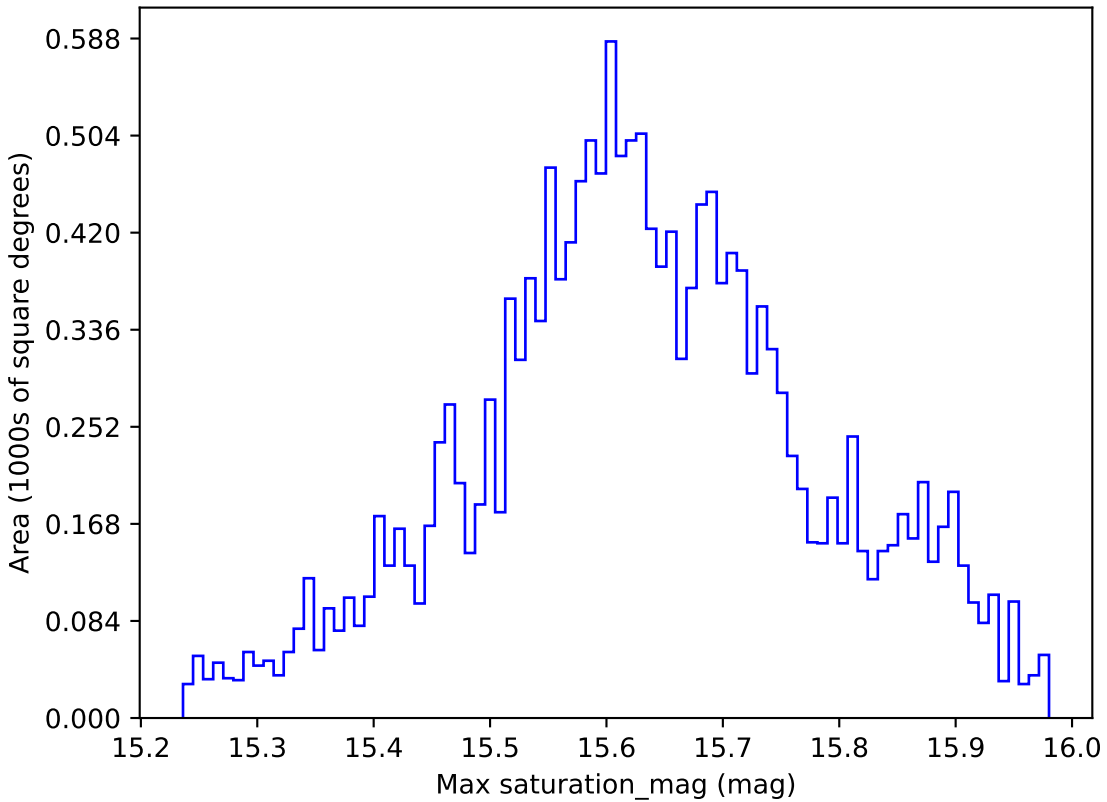
roll_pause_mjdp0_v3.4_10yrs WFD i band: Max saturation_mag
