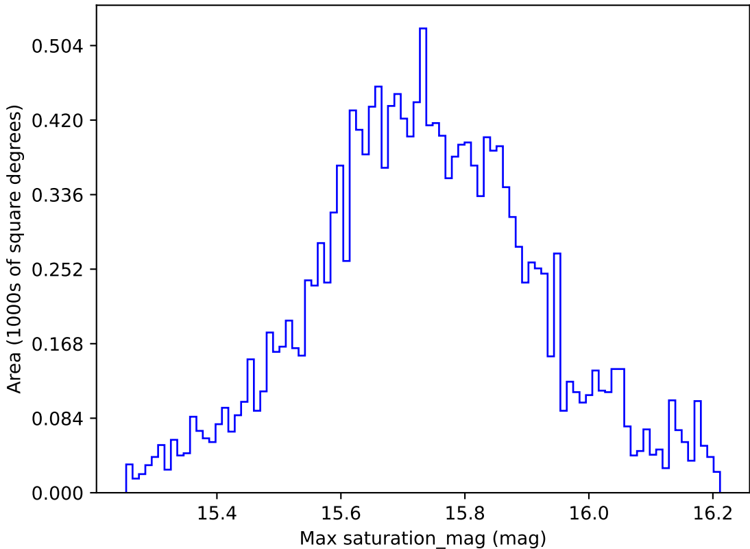
roll_pause_mjdp0_v3.4_10yrs WFD g band: Max saturation_mag
