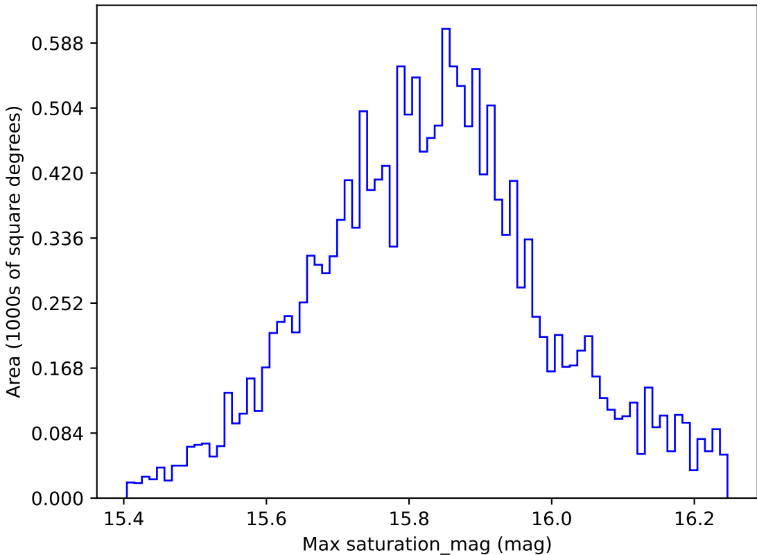
roll_pause_mjdp0_v3.4_10yrs WFD all bands: Max saturation_mag
