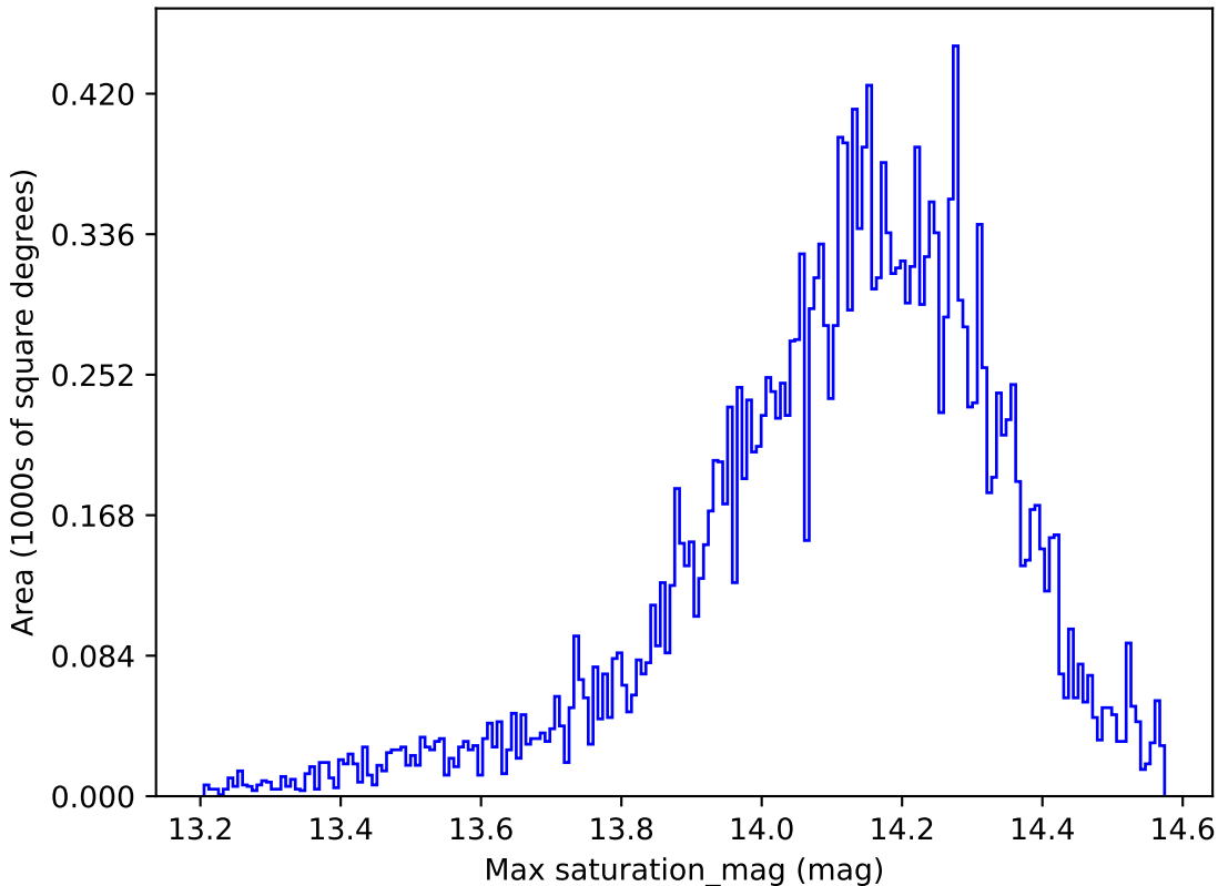
roll_pause_mjdp0_v3.4_10yrs All sky y band: Max saturation_mag
