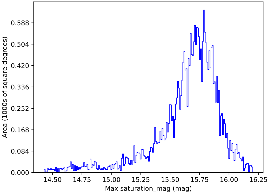
roll_pause_mjdp0_v3.4_10yrs All sky r band: Max saturation_mag
