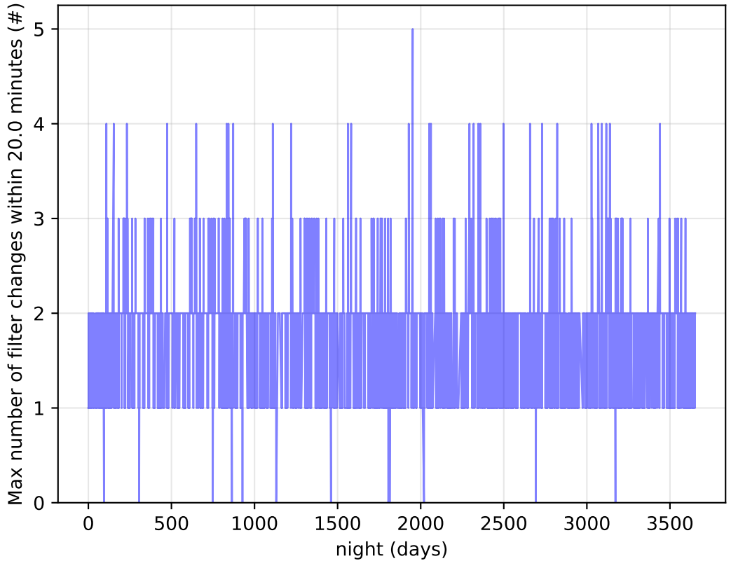
roll_pause_mjdp0_v3.4_10yrs Per Night: Max number of filter changes within 20.0 minutes
