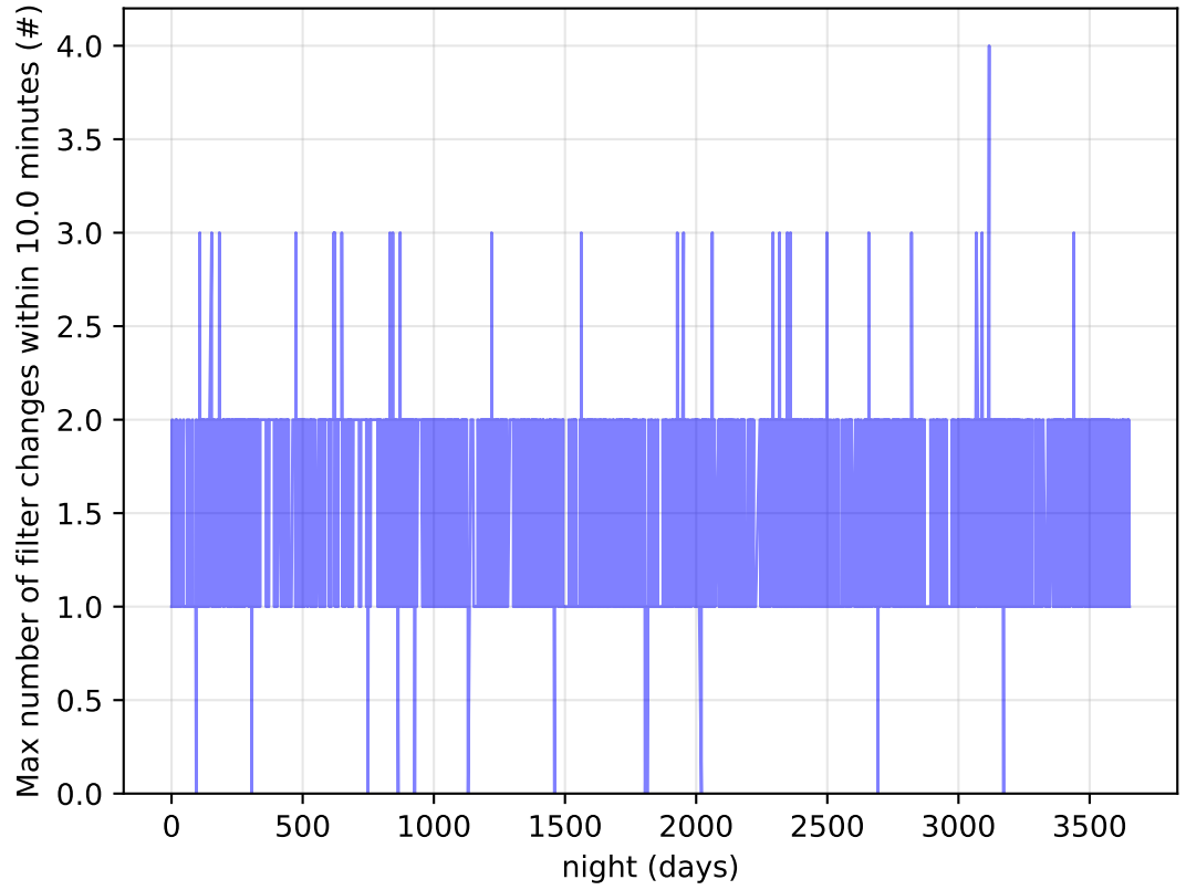
roll_pause_mjdp0_v3.4_10yrs Per Night: Max number of filter changes within 10.0 minutes
