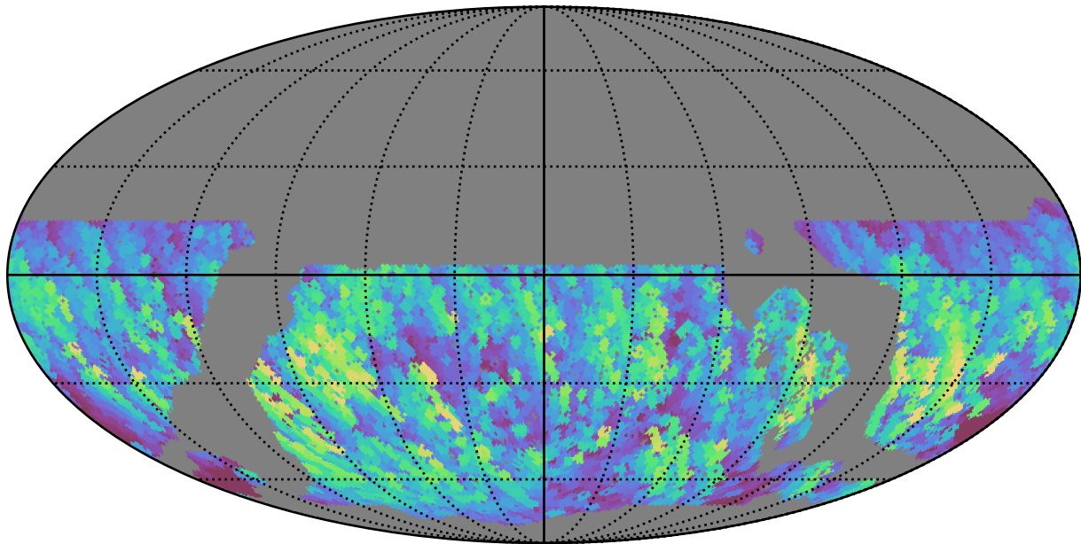
roll_pause_mjdp0_v3.4_10yrs WFD y band: Max normairmass
