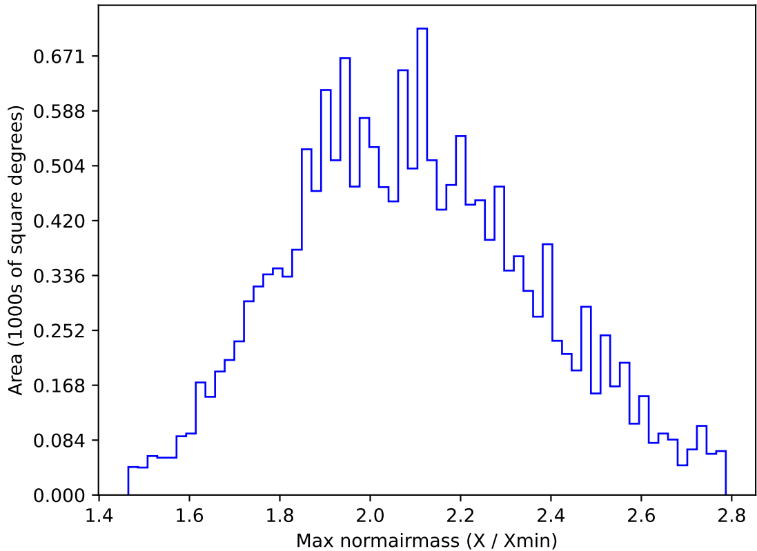
roll_pause_mjdp0_v3.4_10yrs WFD y band: Max normairmass
