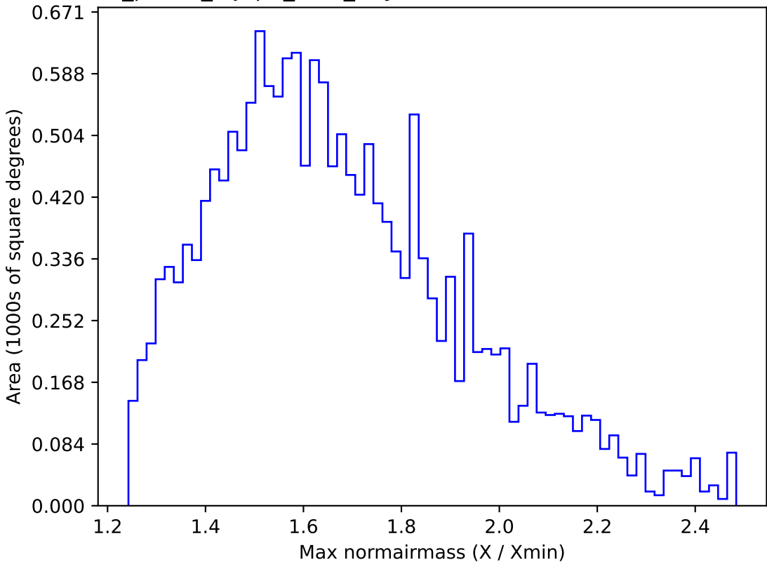
roll_pause_mjdp0_v3.4_10yrs WFD u band: Max normairmass
