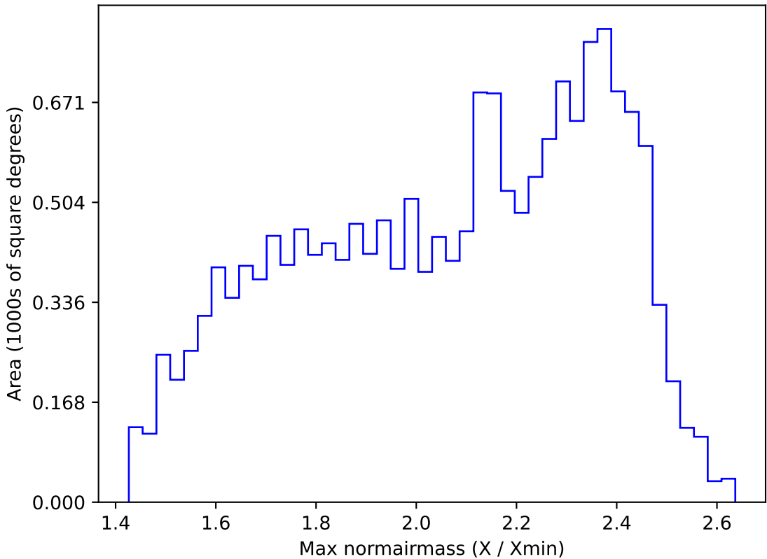
roll_pause_mjdp0_v3.4_10yrs WFD r band: Max normairmass
