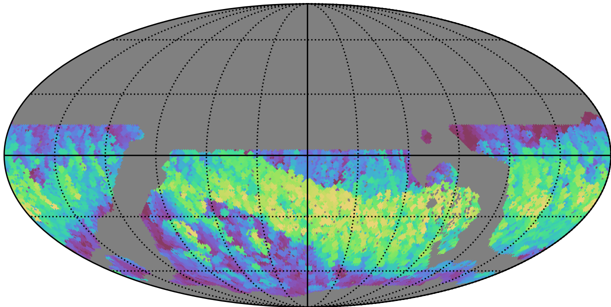
roll_pause_mjdp0_v3.4_10yrs WFD i band: Max normairmass
