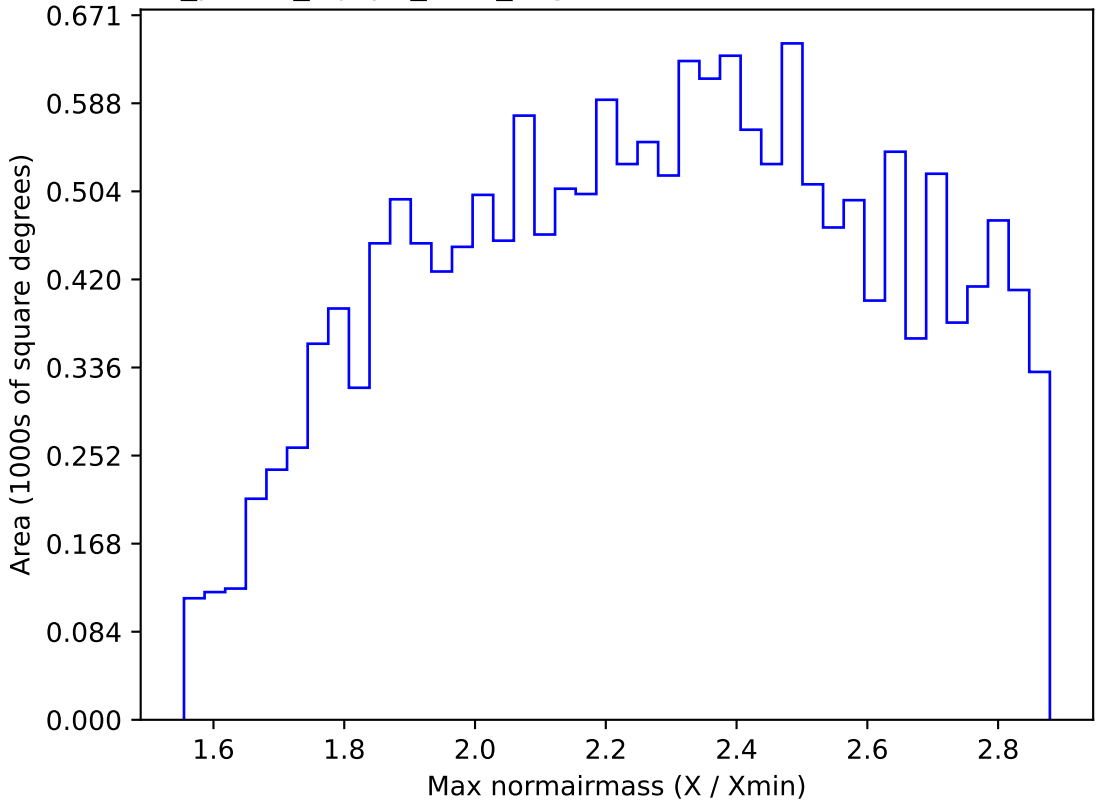
roll_pause_mjdp0_v3.4_10yrs WFD i band: Max normairmass
