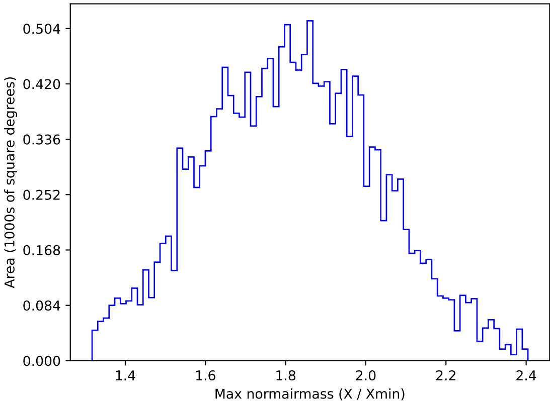
roll_pause_mjdp0_v3.4_10yrs WFD g band: Max normairmass
