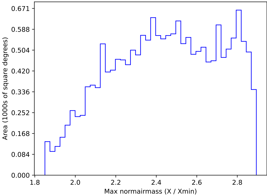
roll_pause_mjdp0_v3.4_10yrs WFD all bands: Max normairmass
