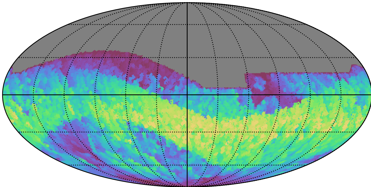
roll_pause_mjdp0_v3.4_10yrs All sky z band: Max normairmass
