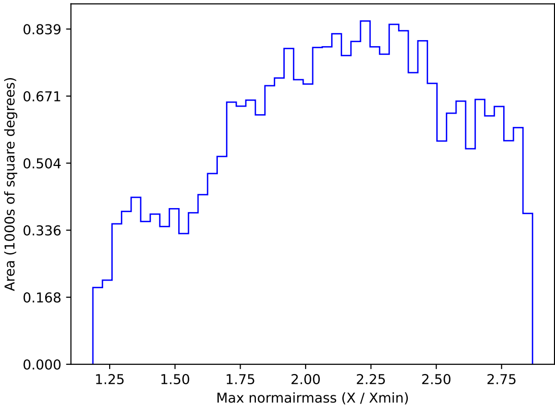
roll_pause_mjdp0_v3.4_10yrs All sky z band: Max normairmass
