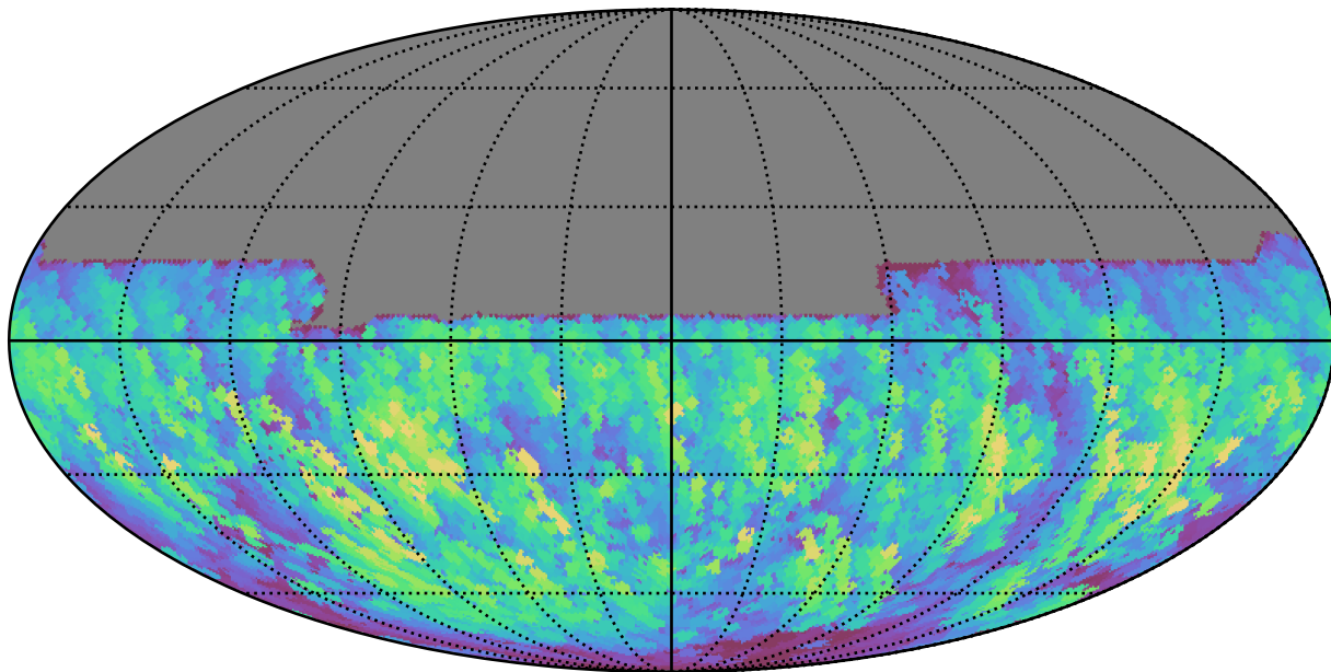
roll_pause_mjdp0_v3.4_10yrs All sky y band: Max normairmass
