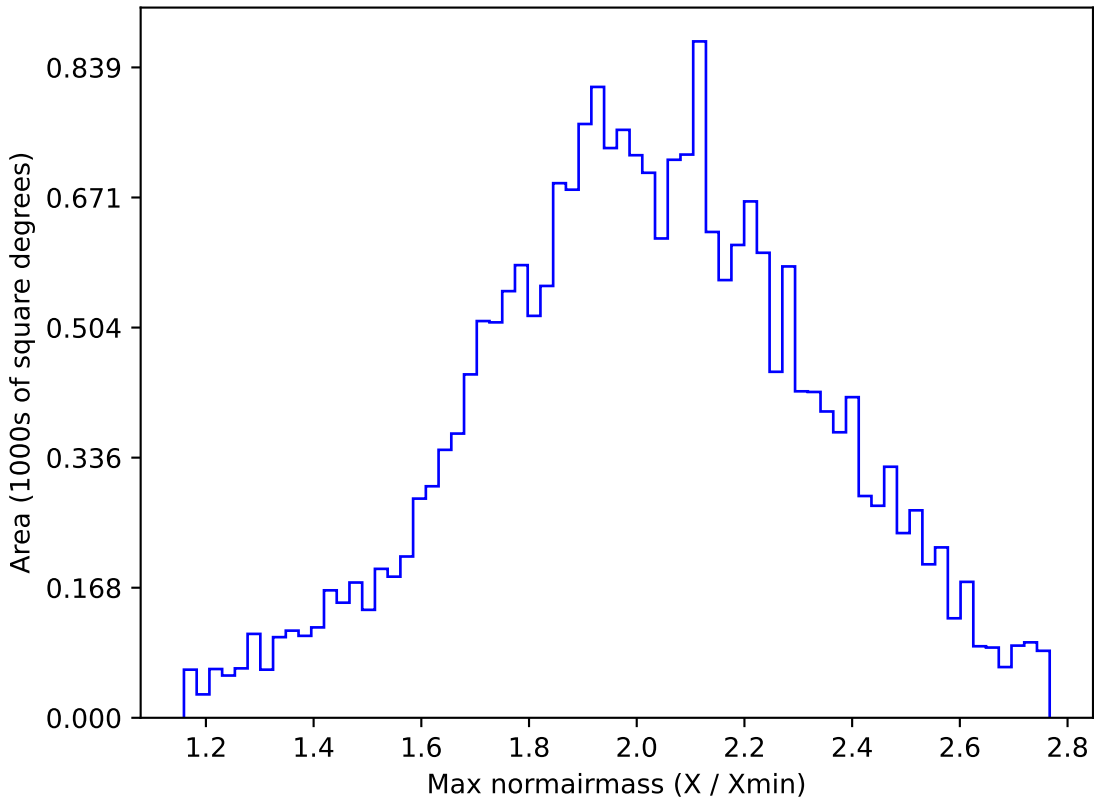
roll_pause_mjdp0_v3.4_10yrs All sky y band: Max normairmass
