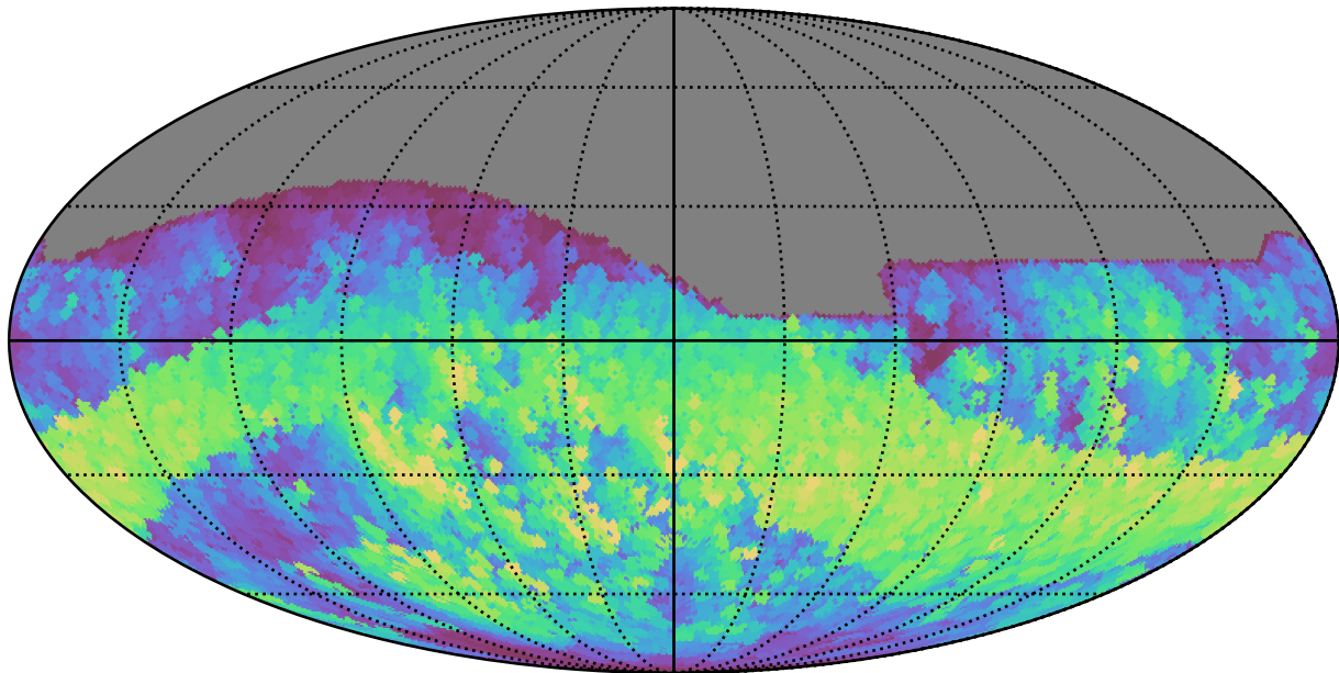
roll_pause_mjdp0_v3.4_10yrs All sky r band: Max normairmass
