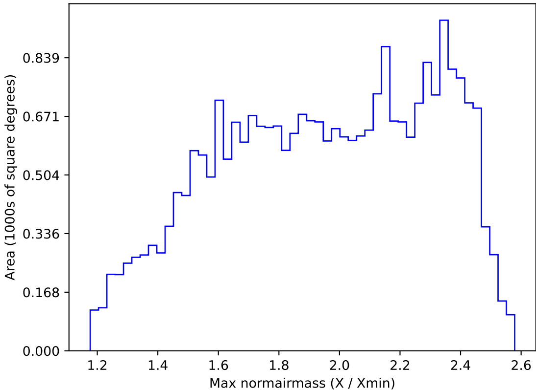
roll_pause_mjdp0_v3.4_10yrs All sky r band: Max normairmass
