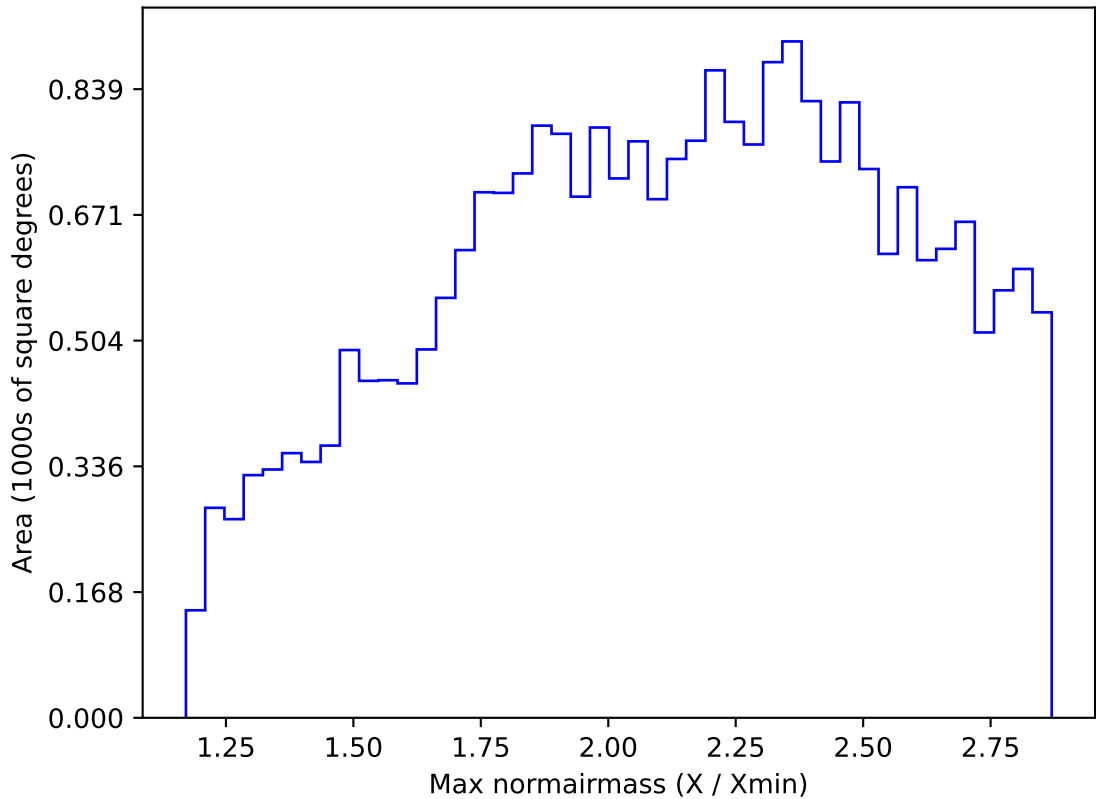
roll_pause_mjdp0_v3.4_10yrs All sky i band: Max normairmass
