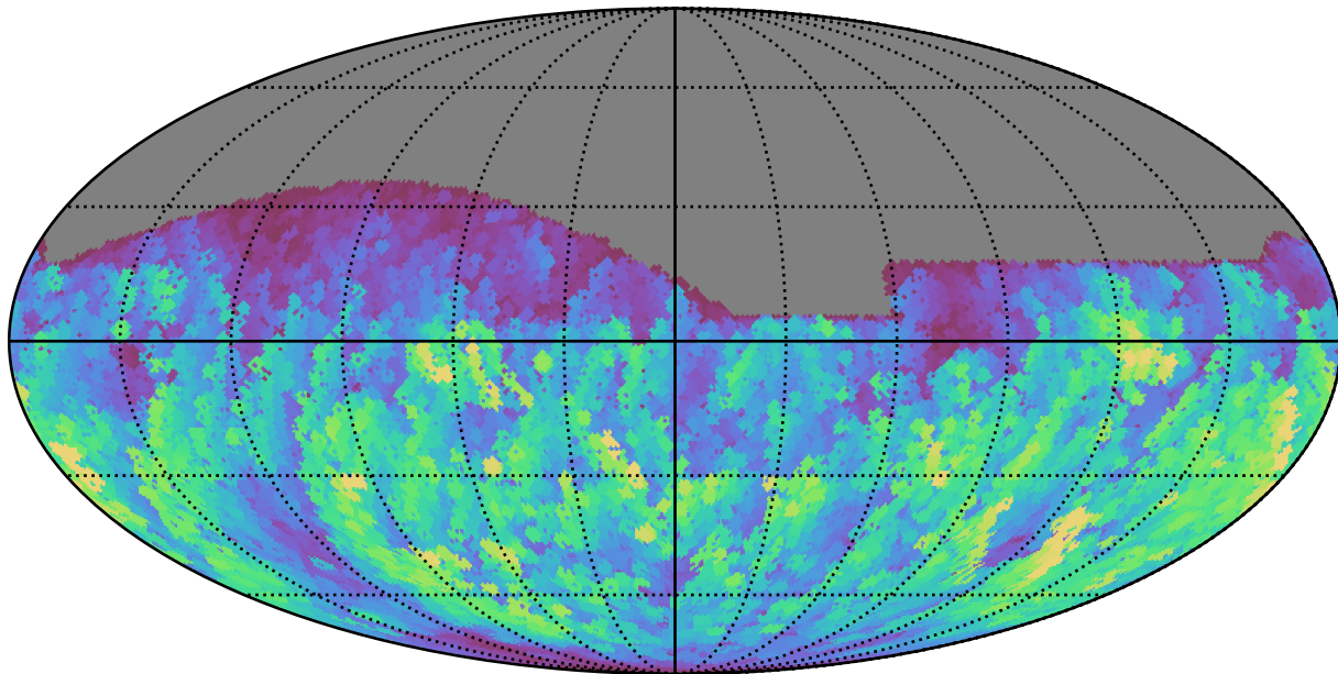
roll_pause_mjdp0_v3.4_10yrs All sky g band: Max normairmass
