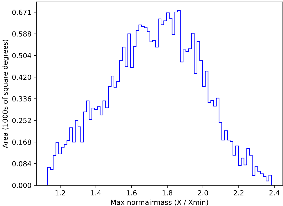
roll_pause_mjdp0_v3.4_10yrs All sky g band: Max normairmass
