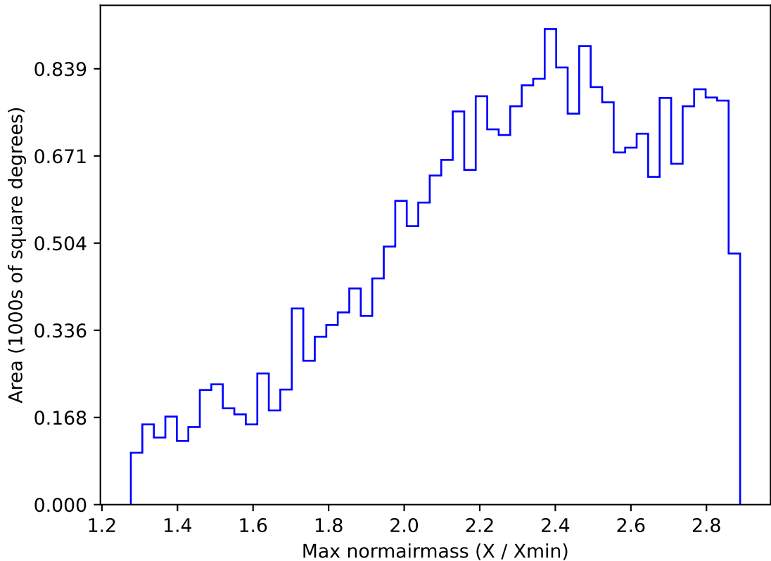
roll_pause_mjdp0_v3.4_10yrs All sky all bands: Max normairmass
