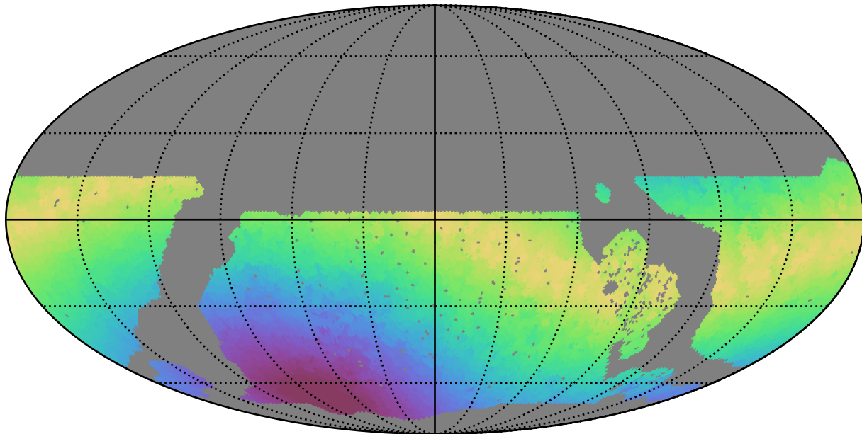
roll_pause_mjdp0_v3.4_10yrs WFD z band: Max moonDistance
