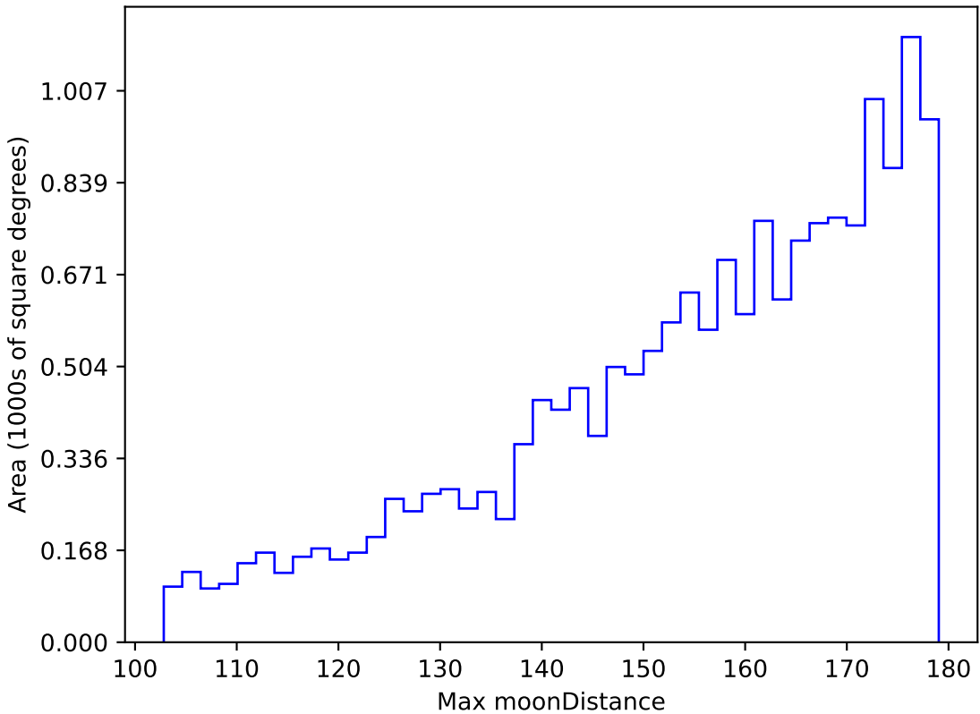
roll_pause_mjdp0_v3.4_10yrs WFD z band: Max moonDistance
