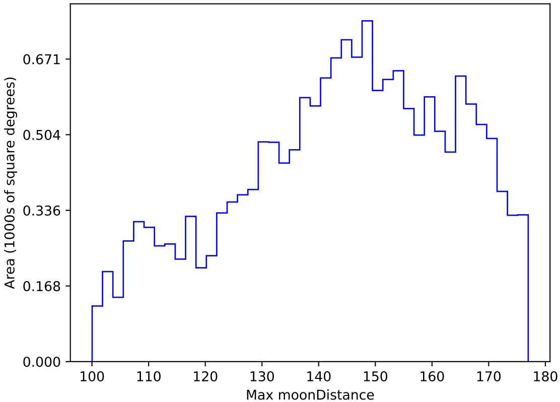
roll_pause_mjdp0_v3.4_10yrs WFD y band: Max moonDistance
