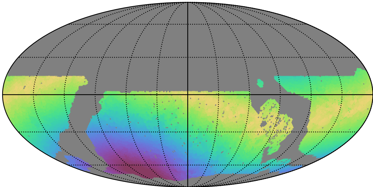
roll_pause_mjdp0_v3.4_10yrs WFD u band: Max moonDistance
