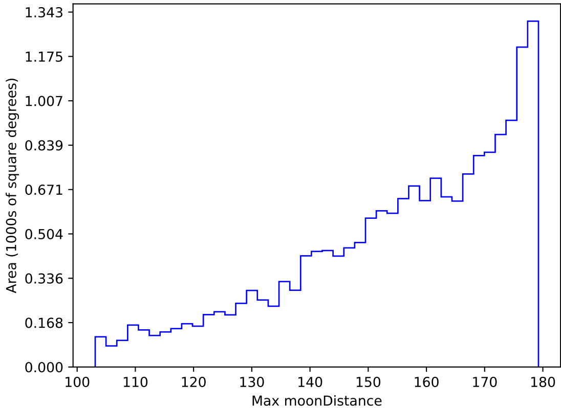
roll_pause_mjdp0_v3.4_10yrs WFD i band: Max moonDistance
