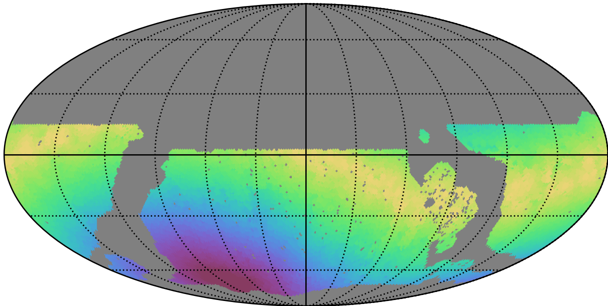
roll_pause_mjdp0_v3.4_10yrs WFD g band: Max moonDistance
