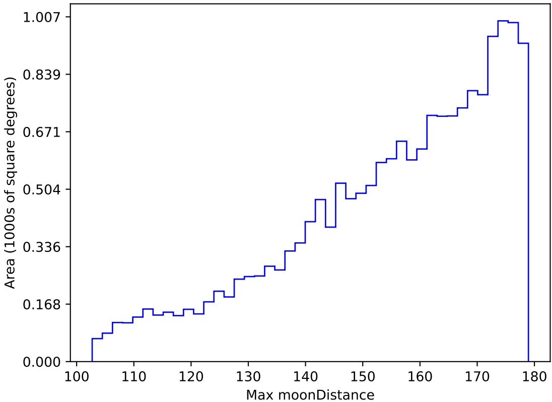
roll_pause_mjdp0_v3.4_10yrs WFD g band: Max moonDistance
