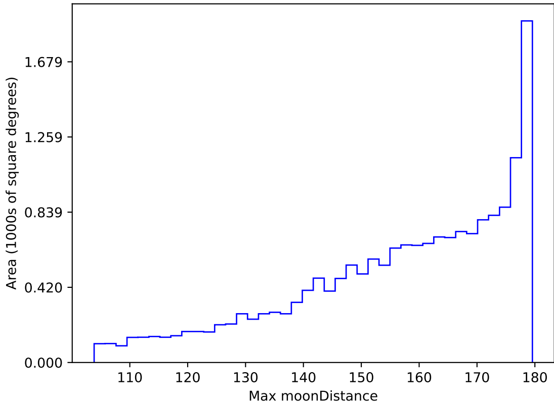
roll_pause_mjdp0_v3.4_10yrs WFD all bands: Max moonDistance
