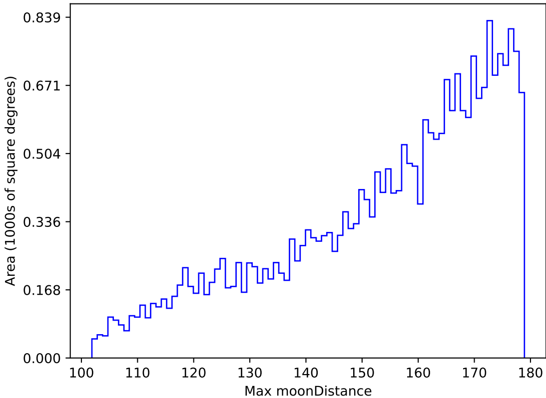
roll_pause_mjdp0_v3.4_10yrs All sky z band: Max moonDistance
