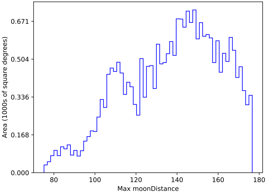
roll_pause_mjdp0_v3.4_10yrs All sky y band: Max moonDistance
