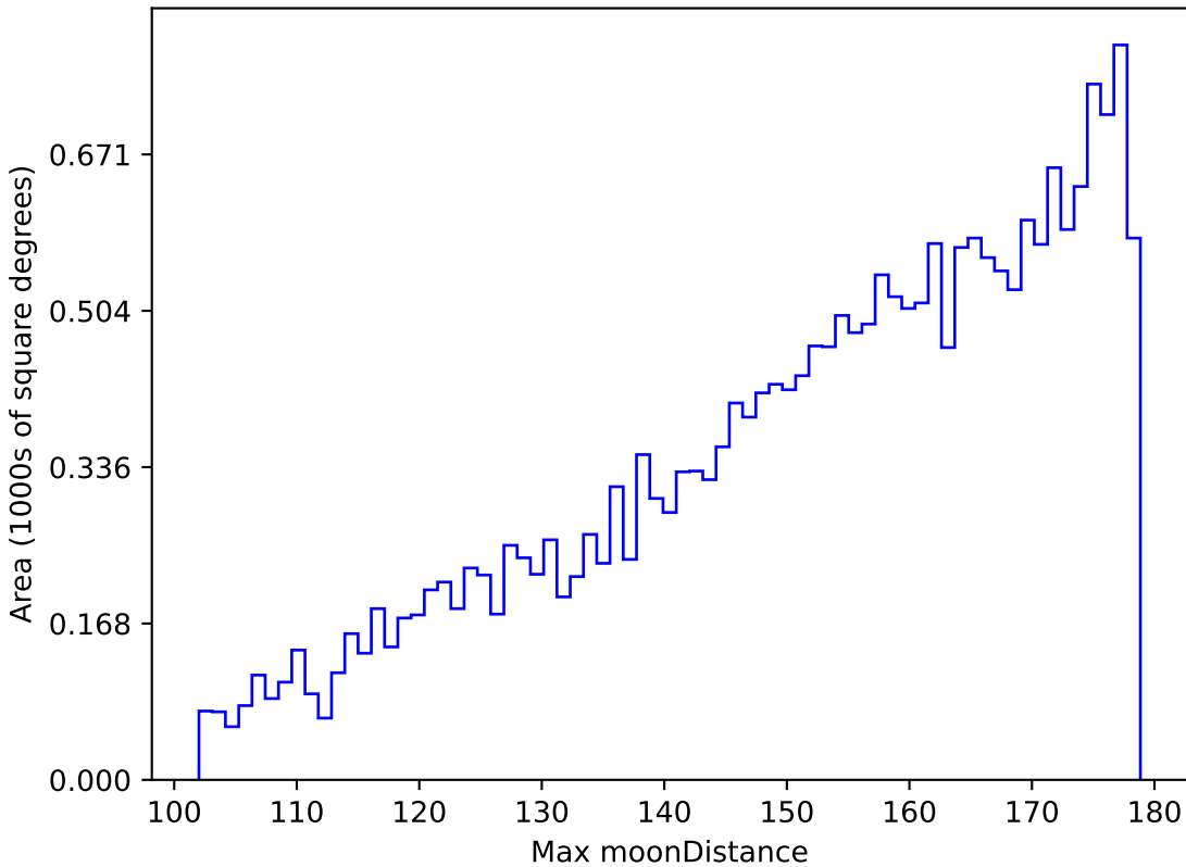
roll_pause_mjdp0_v3.4_10yrs All sky u band: Max moonDistance
